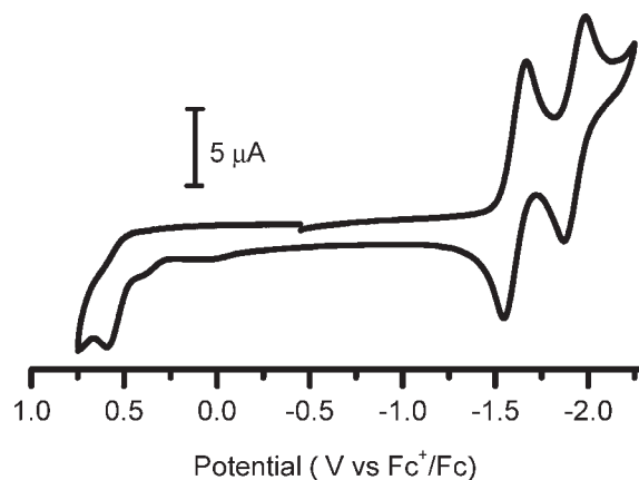
Figure 4. CV of 4 in a 0.1 M dichloromethane/(Bu 4 N)(PF 6 ) solution. The scan rate is 100 mV s -1 .
